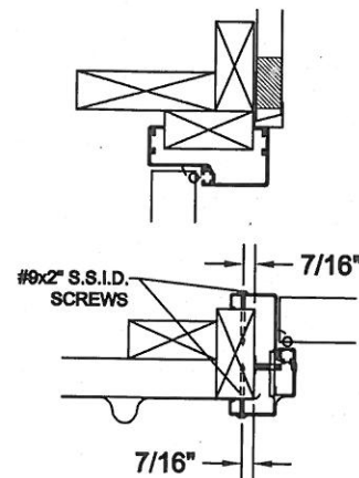
INSWING DETAILS
