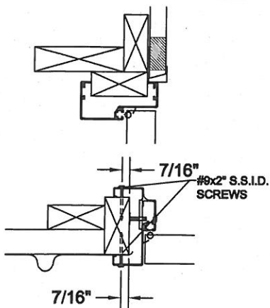
OUTSWING DETAILS
