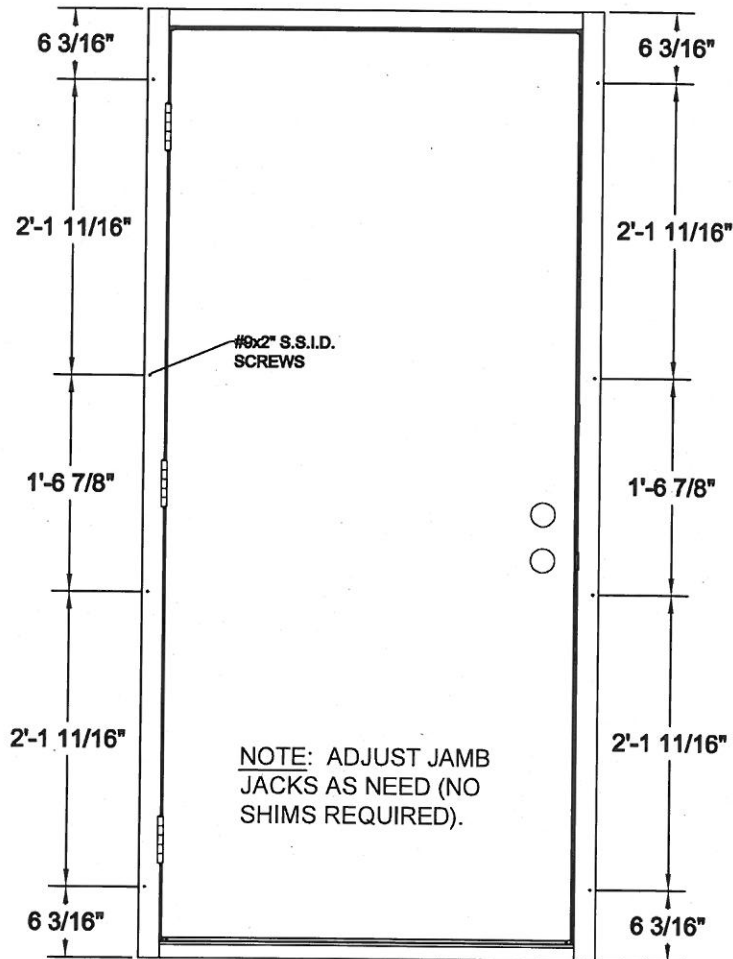
OUTSWING DETAILS
